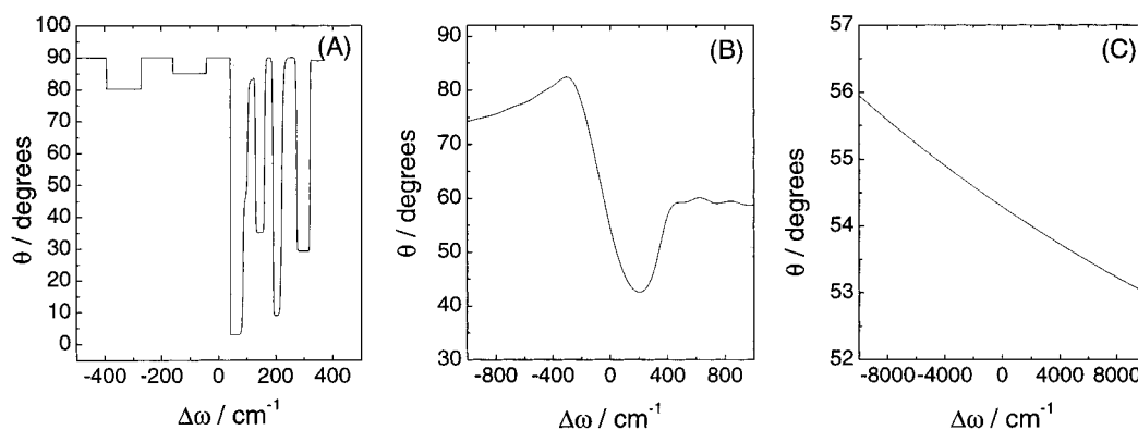
Figure 5. Frequency dependence of \theta , the average angle between the excitonic transition dipole and (OZ)-axis for models (A)–(C) of a helical aggregate consisting of N = 100 RU.
